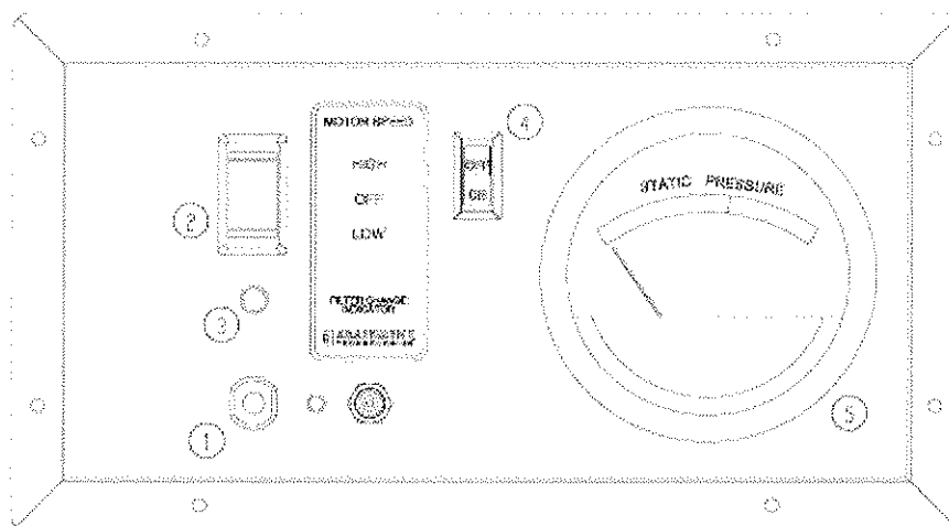
H2KMA Control Panel Drawing
